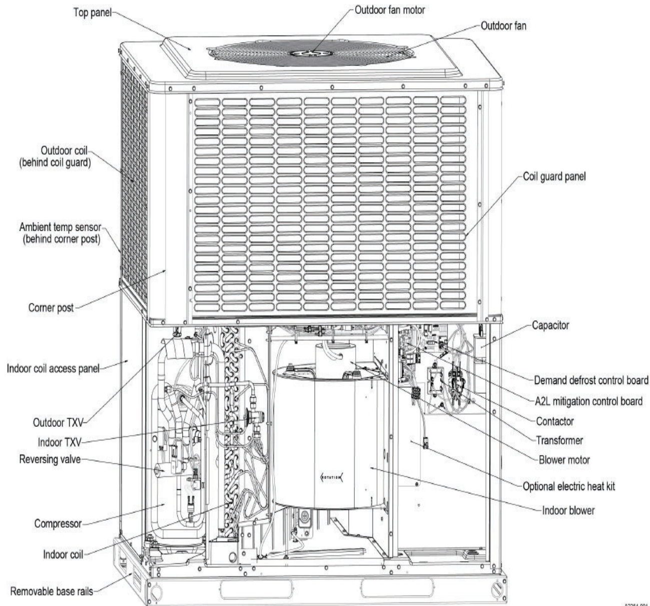
Figure 1: Unit components
